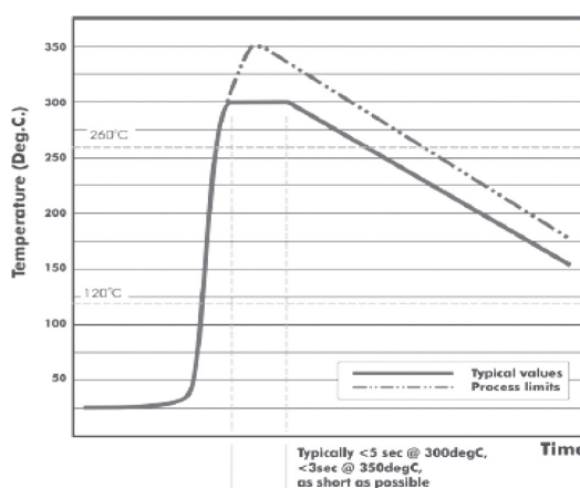
Fig. 4 Recommended soldering profile by manual with SnAgCu series solder.
