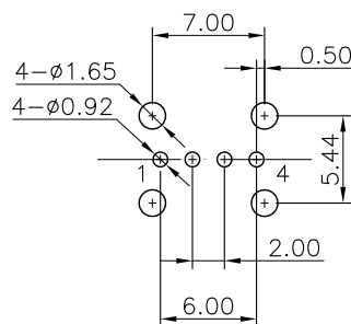
RECOMMENDED PCB LAYOUT TOP VIEW(TOL:±0.05)
