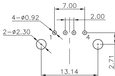
RECOMMENDED PCB LAYOUT TOP VIEW(TOL:±0.05)
