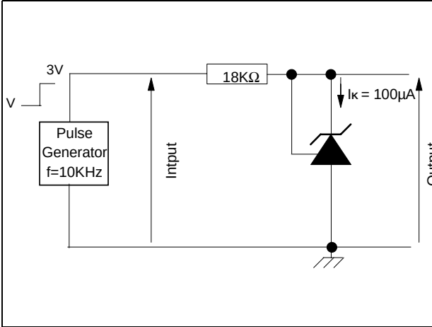
Figure 13. Test circuit for pulse response at I_K=100\mu A
