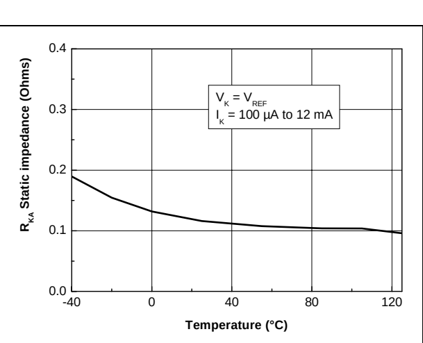
Figure 6. Static impedance vs temperature
