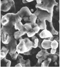
Figure 2. Sintered Tantalum
