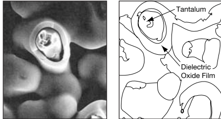
Figure 3. Dielectric Layer
