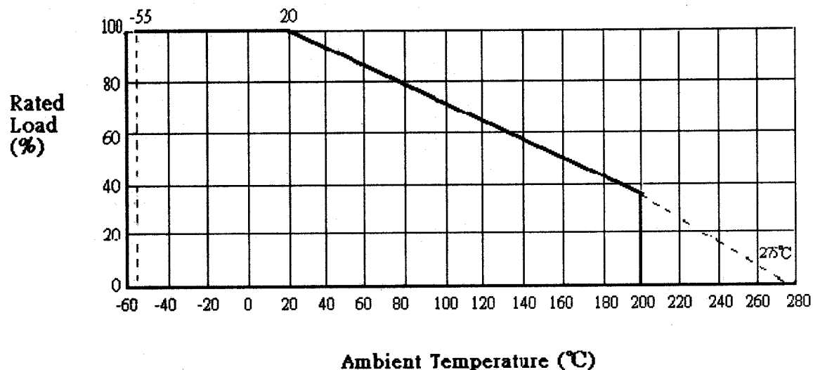
DERATING CURVE
