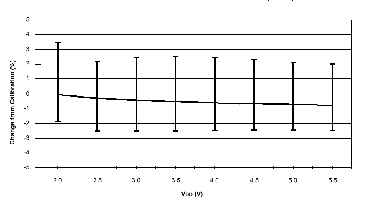
FIGURE 18-41: TYPICAL HFINTOSC FREQUENCY CHANGE vs. V_{DD} ( 125^{\circ}\text{C} )
