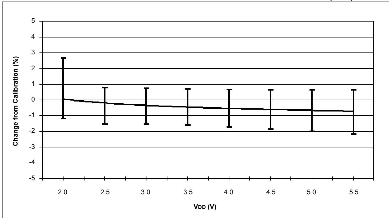
FIGURE 18-40: TYPICAL HFINTOSC FREQUENCY CHANGE OVER DEVICE V_{DD} ( 85^{\circ}\text{C} )
