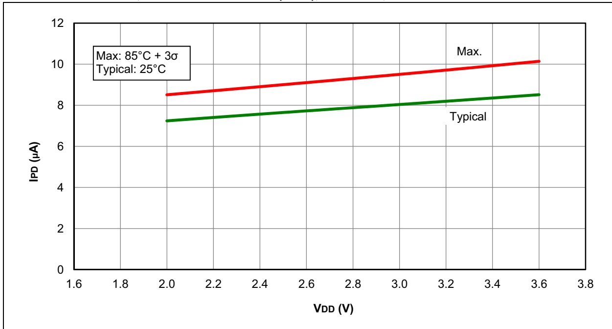
FIGURE 26-28: I_{PD} , BROWN-OUT RESET (BOR), BORV = 1, PIC16LF1507 ONLY
