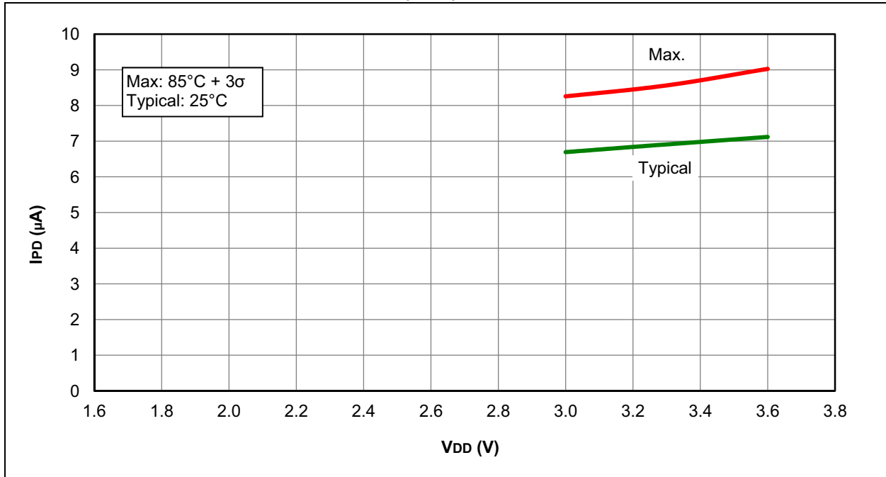
FIGURE 26-27: I_{PD} , BROWN-OUT RESET (BOR), BORV = 0, PIC16LF1507 ONLY
