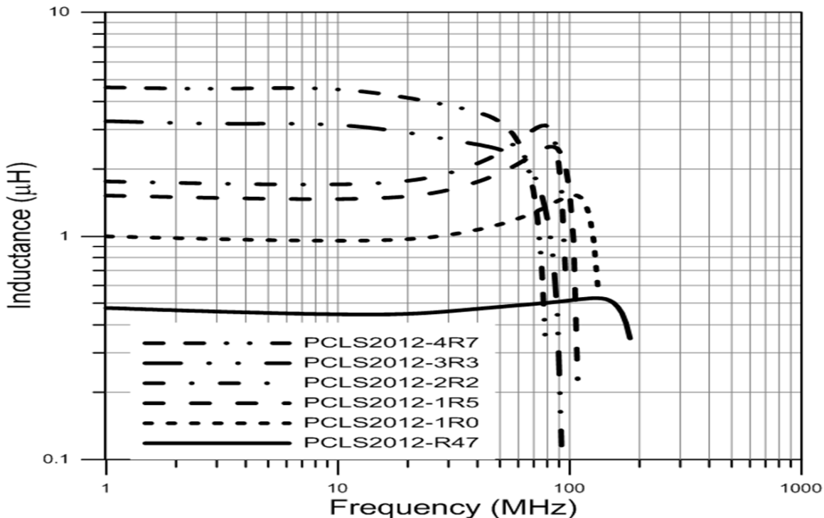
Inductance vs. Frequency
