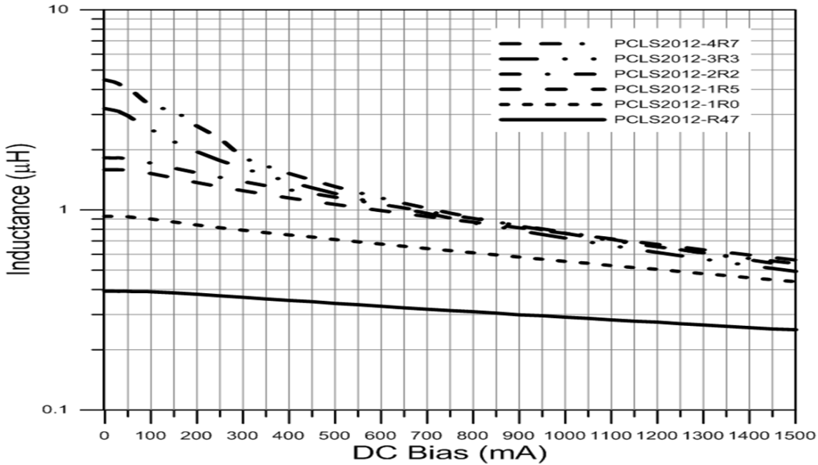
Inductance vs. DC Bias Current
