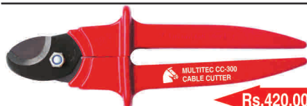
Model No.: CC-300 • For cutting Copper/Aluminium conductor single wire upto 24mm 2 . • Easy cutting with one hand operation due to high transmission ratio. • Material : special high grade alloy steel. • Induction hardened and tempered.
