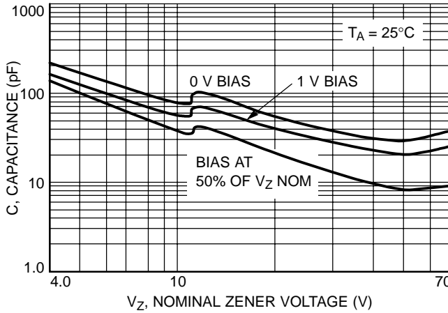
Figure 3. Typical Capacitance
