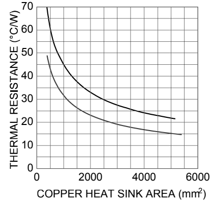
Figure 6. PCB Heat Sink Thermal Resistance
