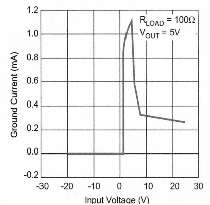
Figure 9. LM29150 Ground Current vs. Input Voltage
