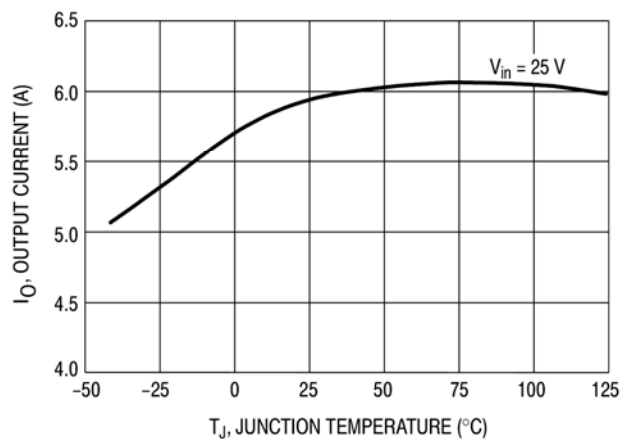
Figure 5. Current Limit
