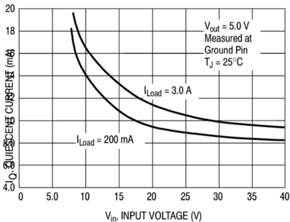
Figure 6. Quiescent Current
