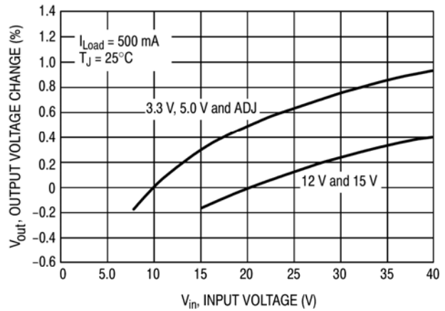
Figure 3. Line Regulation
