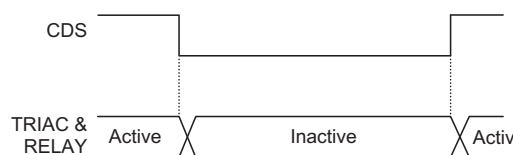
Fig.7 CDS Timing
