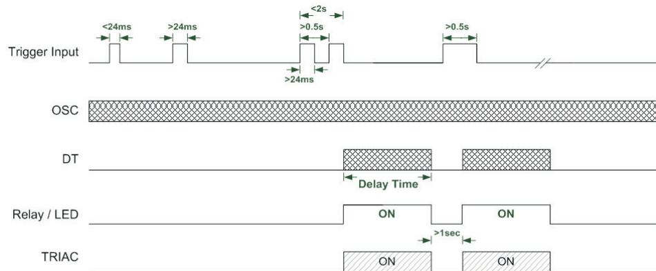
Fig.11 Trigger Timing
