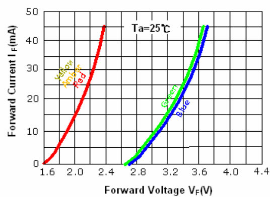
< Figure 7 Forward voltage & forward current for PLCC 3528 series >
