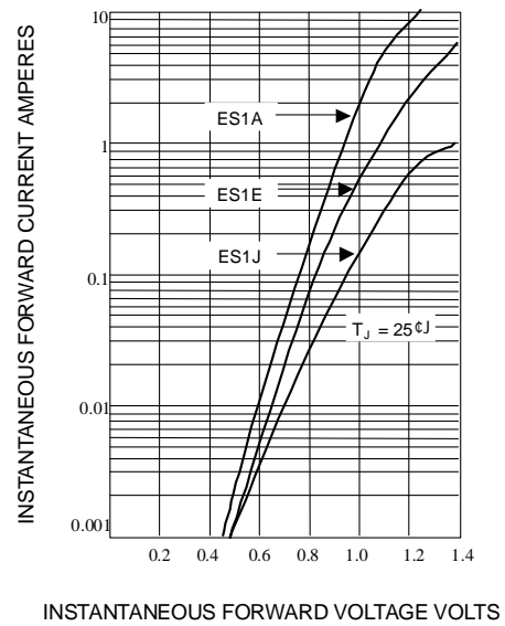
Fig. 4-TYPICAL FORWARD CHARACTERISTICS
