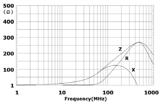
EBMS160808B301
