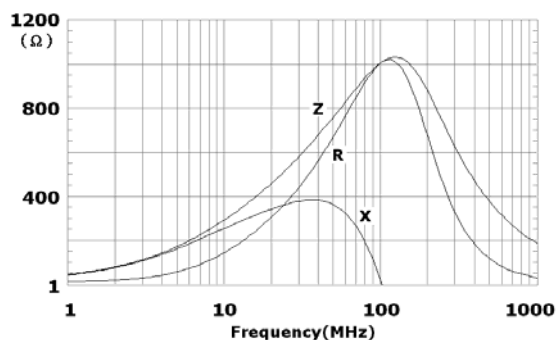
EBMS160808A102
