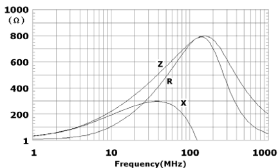
EBMS160808A751
