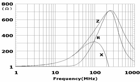
EBMS160808K471
