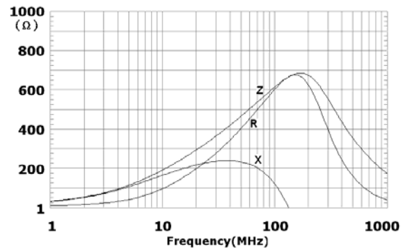
EBMS160808A102
