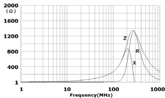
EBMS160808H102
