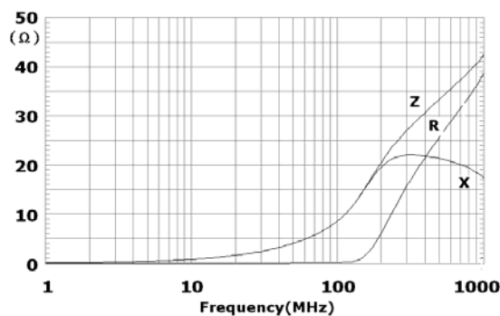
EBMS160808H680
