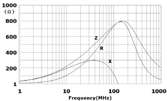
EBMS160808A751
