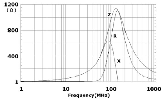
EBMS160808K601
