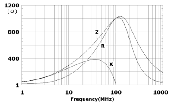
EBMS160808A102
