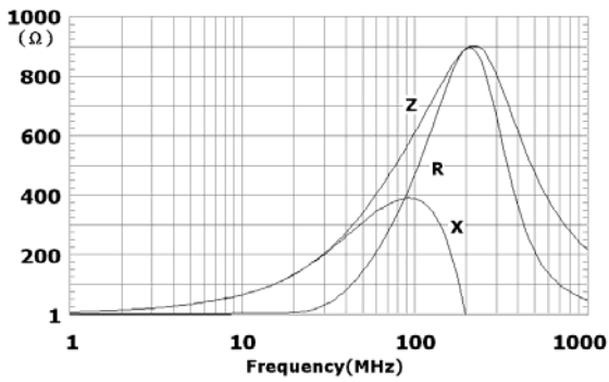
EBMS160808K471
