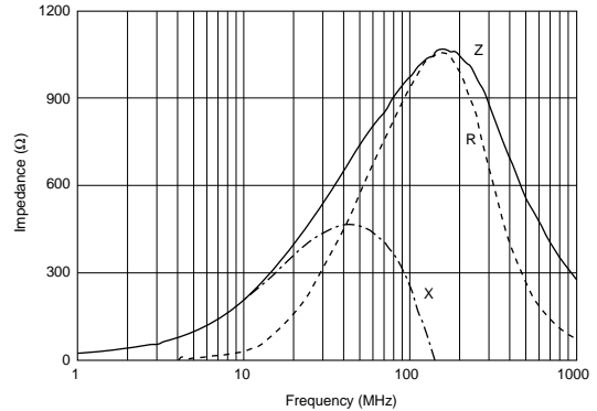
BLM15AG102SN1
