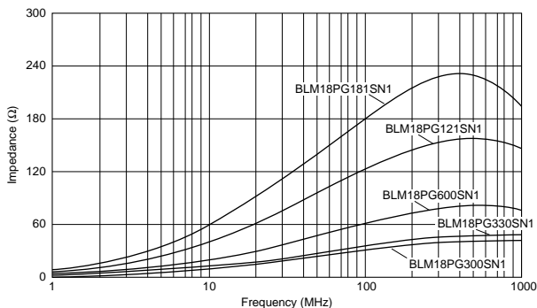
BLM18P Series
