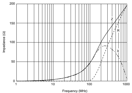
BLM18BB470SN1
