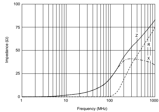
BLM18BB220SN1
