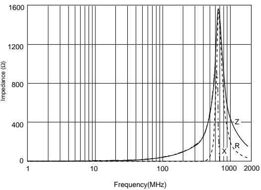
BLM18BA470SN1
