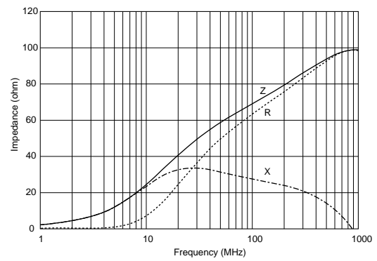
BLM15AG700SN1
