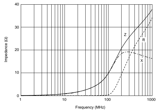
BLM18BB100SN1
