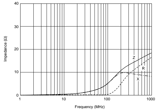
BLM18BB050SN1
