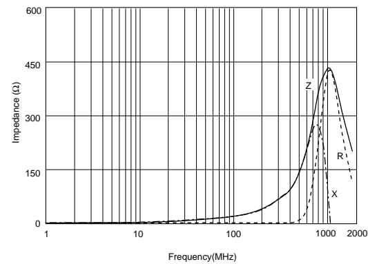
BLM18BA220SN1
