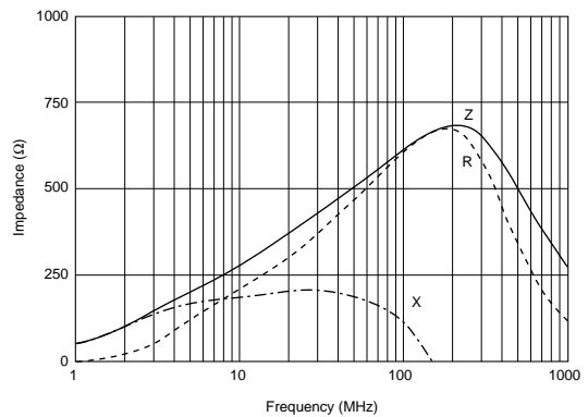
BLM18RK601SN1
