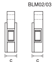
c: Total Thickness of Tape (Paper Tape)
