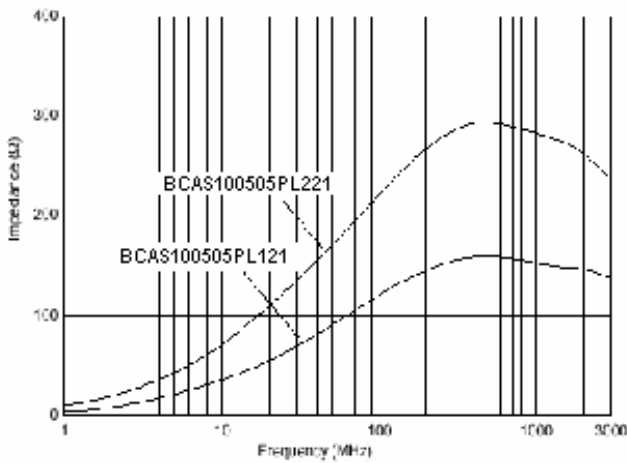
BCAS100505PL SERIES
