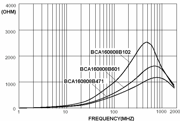
BCAS160808B SERIES
