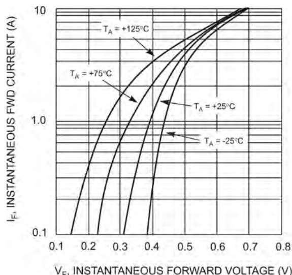
Fig. 2 Typical Forward Characteristics - B320B thru B340B
