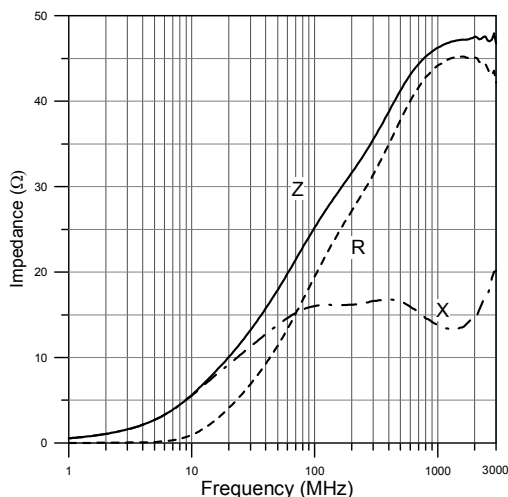
ACMS321611I310 1.5A
