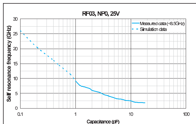
Fig. 3 Self resonance frequency vs. Capacitance (0201 size)
