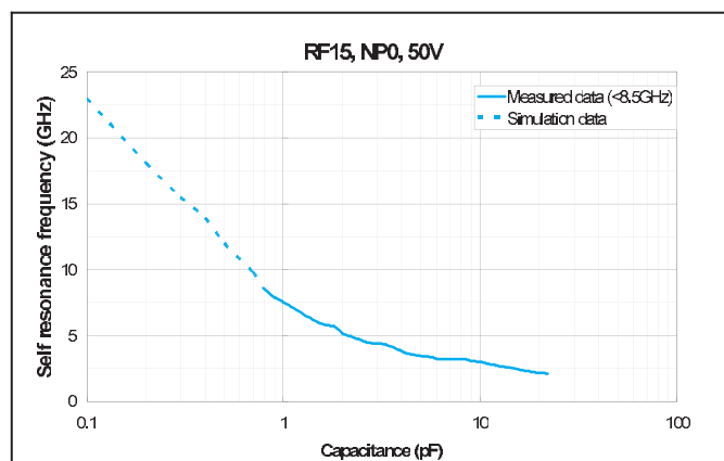
Fig. 4 Self resonance frequency vs. Capacitance (0402 size)
