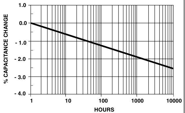
AGING RATE - BX
