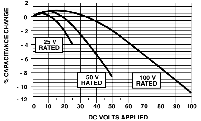
VOLTAGE COEFFICIENT OF CAPACITANCE - BX
